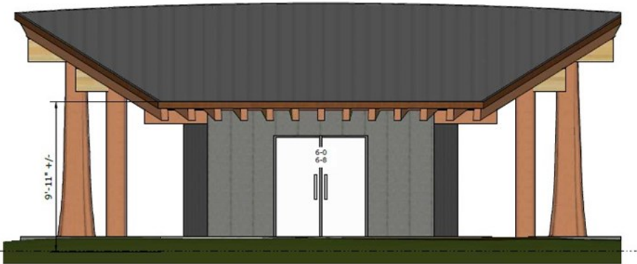
East Elevation scale 3/16"=1'-0"
