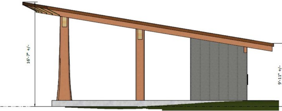
South Elevation scale 3/16"=1'-0"
