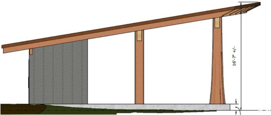
North Elevation scale 3/16"=1'-0"
