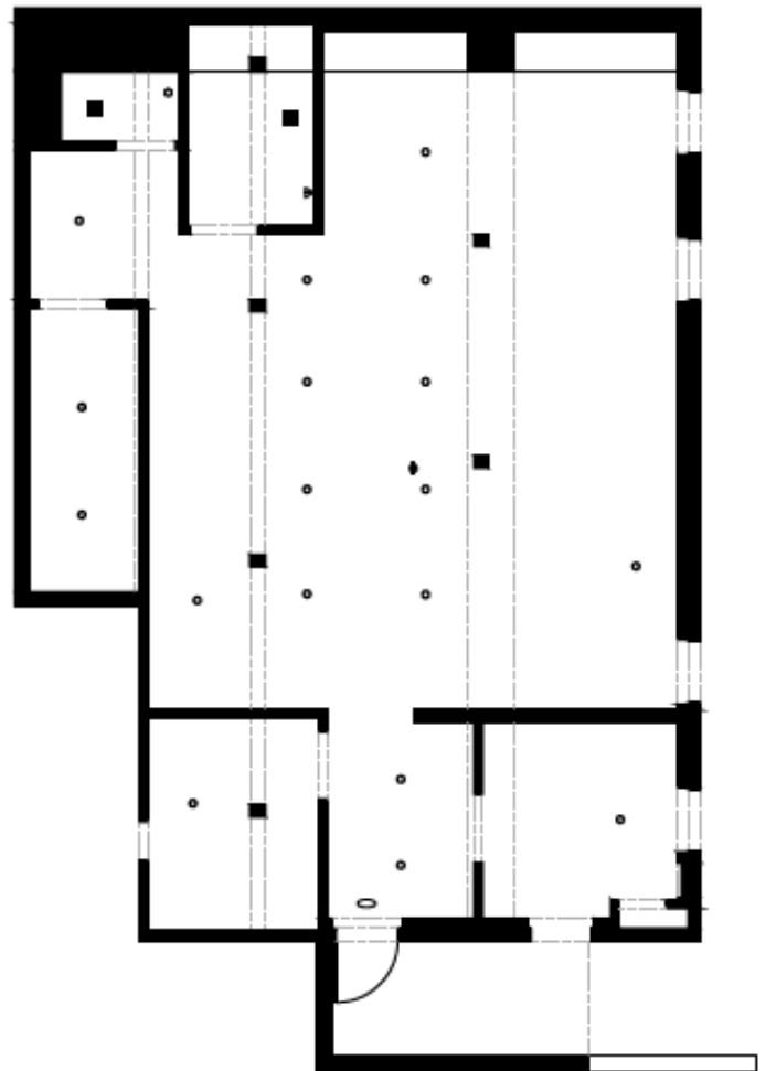
2. REFLECTED CEILING PLAN
